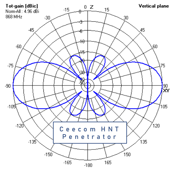
2D radiation pattern looking in from side (slice)
