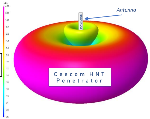
3D image of radiation pattern
