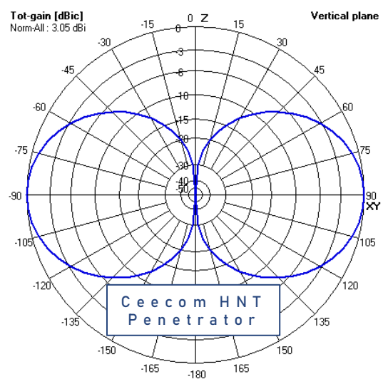
V Plane Pattern 60° - Looking in from the side
