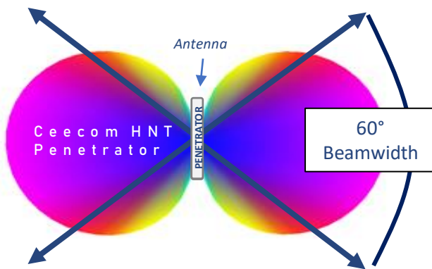
H Plane Pattern 360° - Looking down from above
