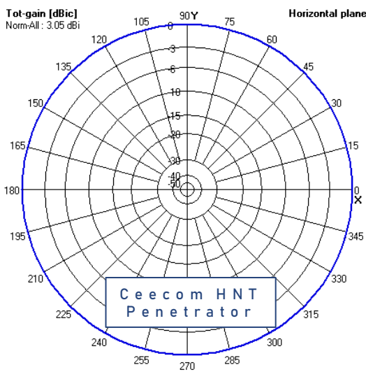
H Plane Pattern 360° - Looking down from above
