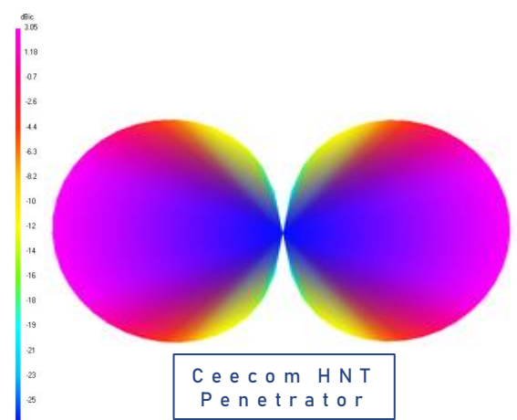
2D radiation pattern looking in from side (slice)
