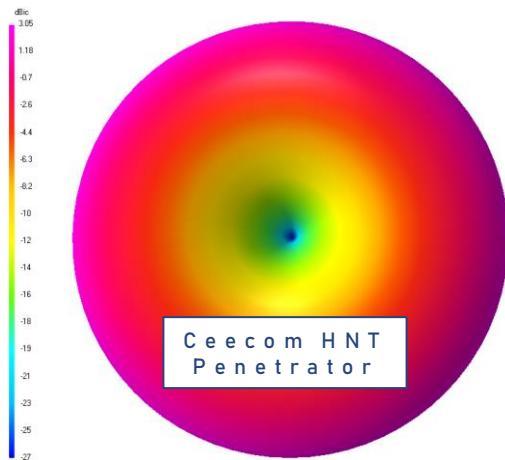
3D radiation pattern looking down from above
