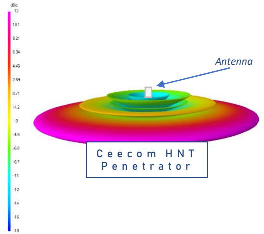
3D image of radiation pattern
