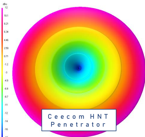
3D radiation pattern looking down from above
